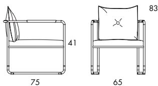
O652 14.5 kg | 0.45 m 3 /pc (1.7 m 3 /4 pcs)
